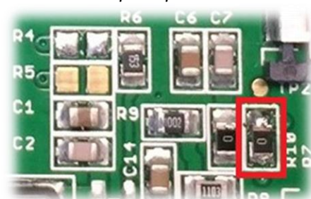
Jumper Option #2
