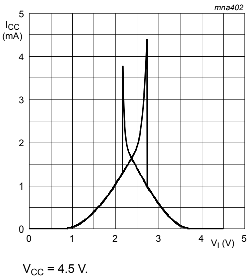
Fig. 11. Typical 74AHC3G14 transfer characteristics
