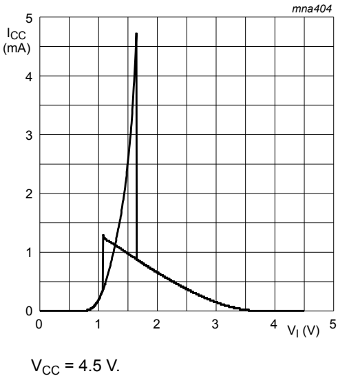
Fig. 13. Typical 74AHCT3G14 transfer characteristics
