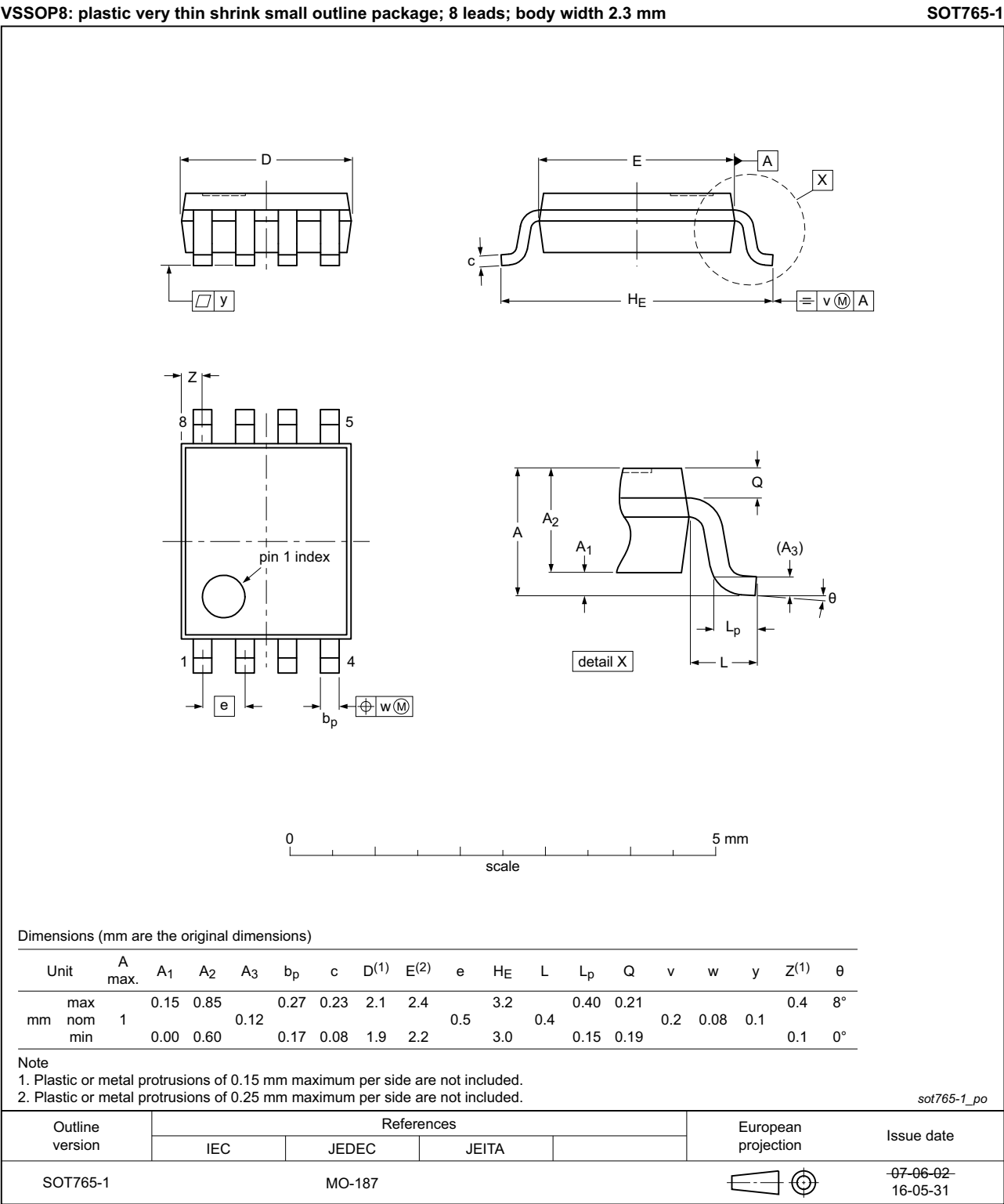
Fig 12. Package outline SOT765-1 (VSSOP8)
