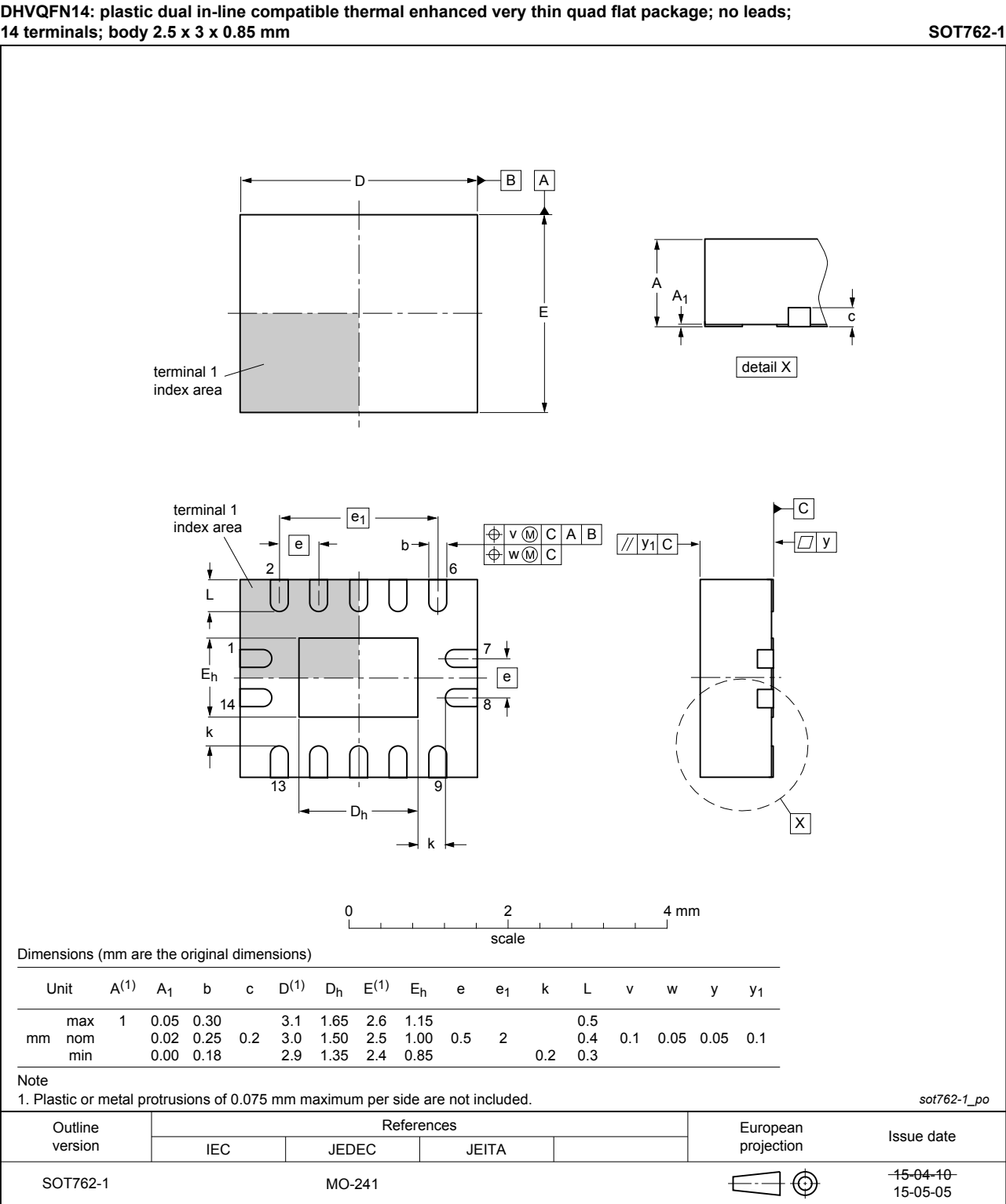
Figure 13. Package outline SOT762-1 (DHVQFN14)
