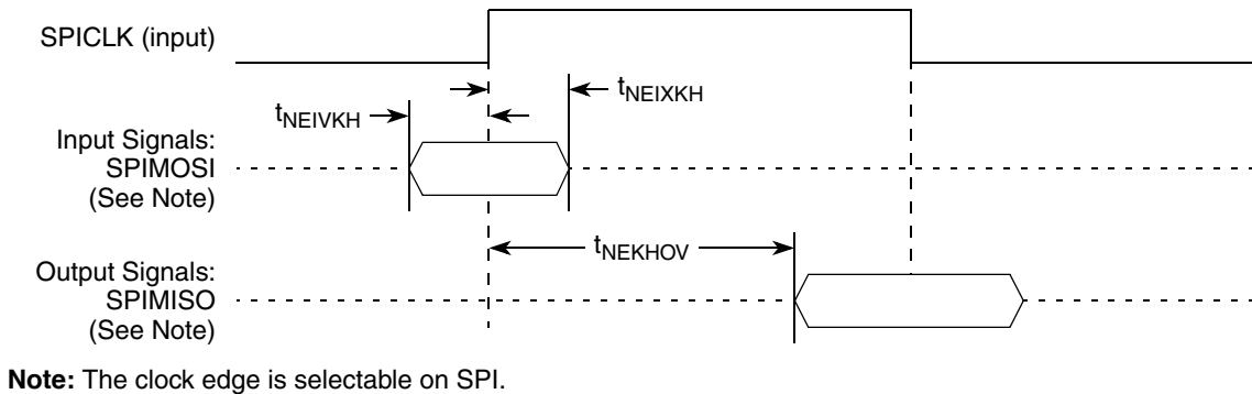
Figure 50. SPI AC Timing in Slave Mode (External Clock) Diagram
