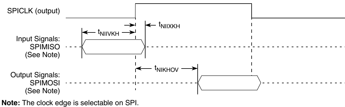
Figure 51. SPI AC Timing in Master Mode (Internal Clock) Diagram
