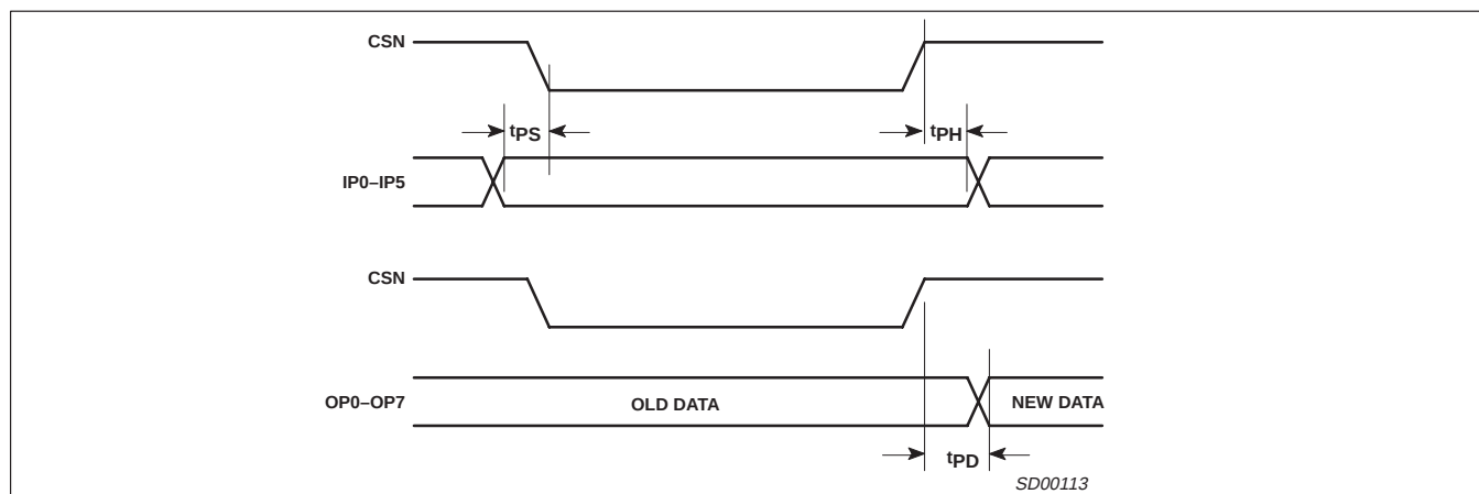
Figure 7. Port Timing
