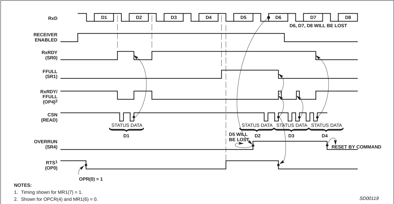
Figure 13. Receive timing
