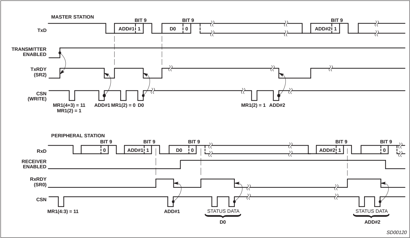
Figure 14. Wake-up mode
