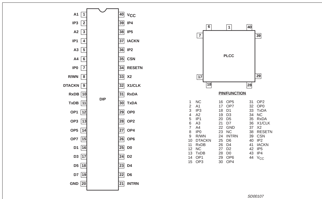
Figure 1. Pin Configurations
