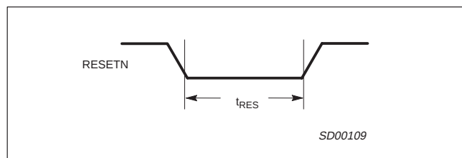
Figure 3. Reset Timing
