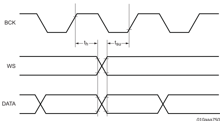
Fig 4. I 2 S timing
