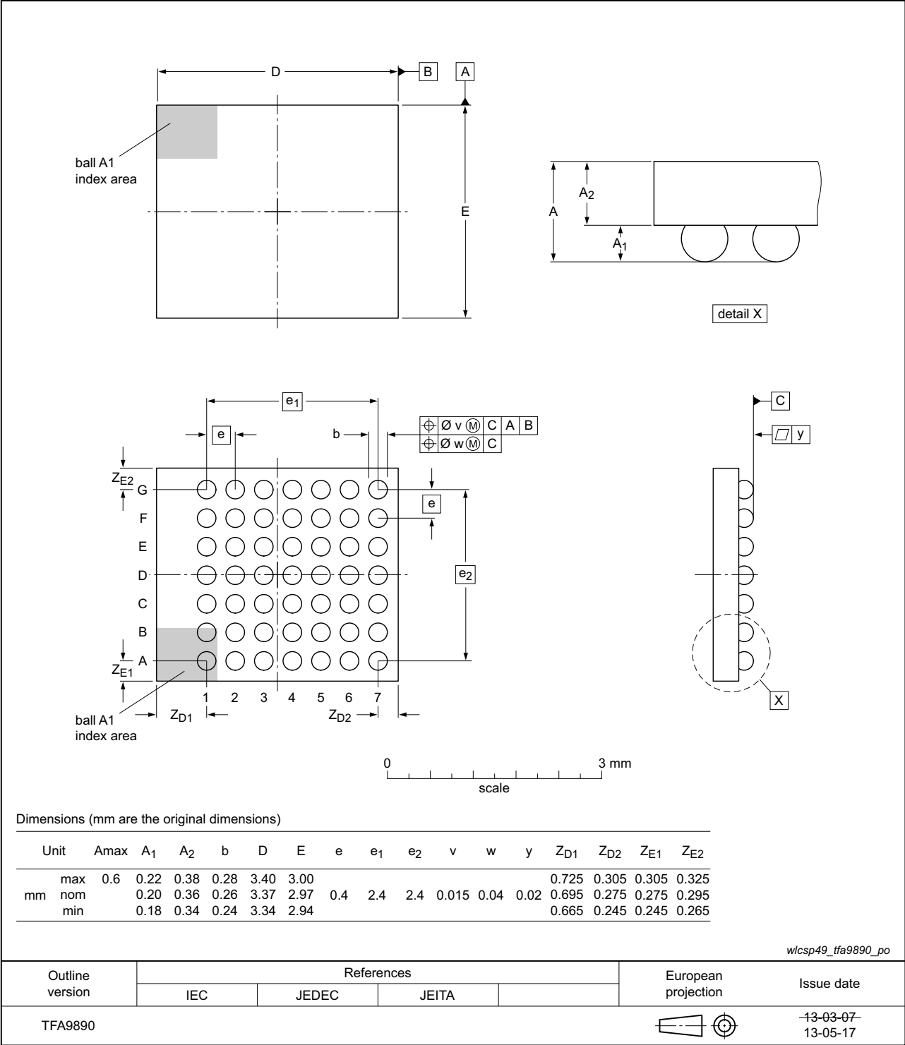
Fig 15. Package outline TFA9890 (WLCSP49)
