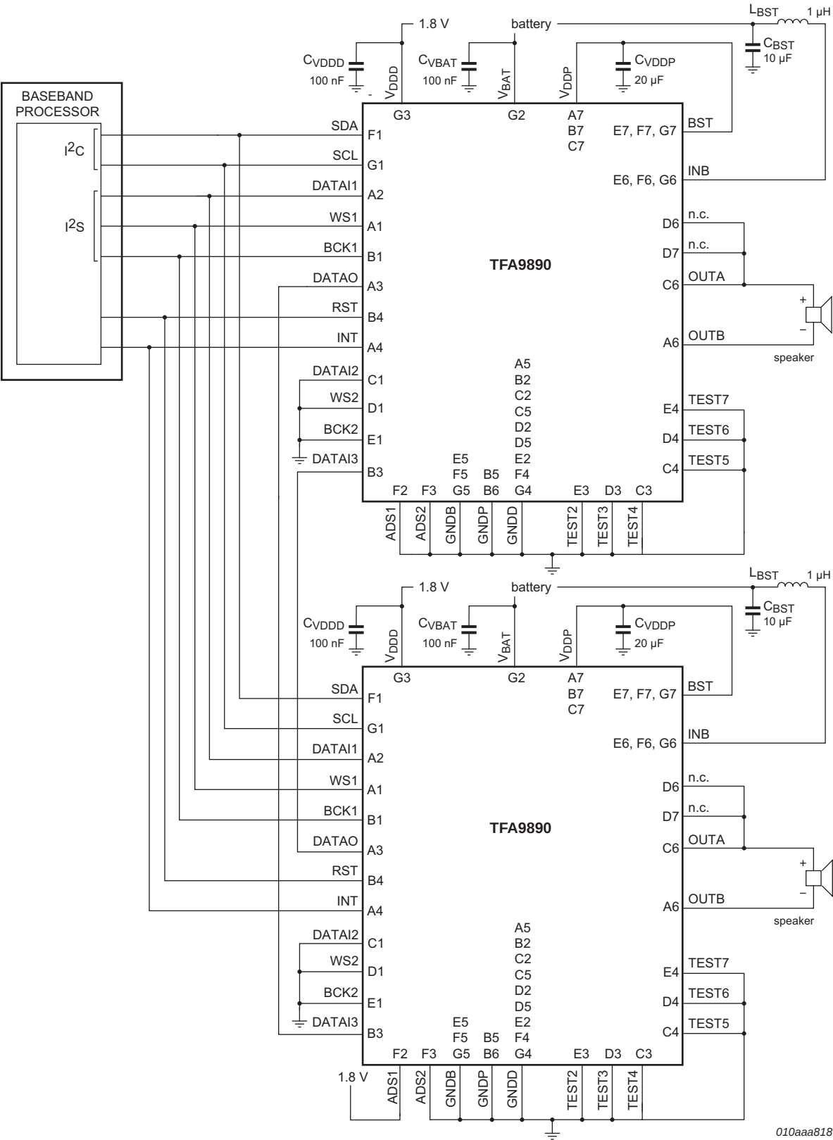
Fig 7. Typical stereo application (simplified)
