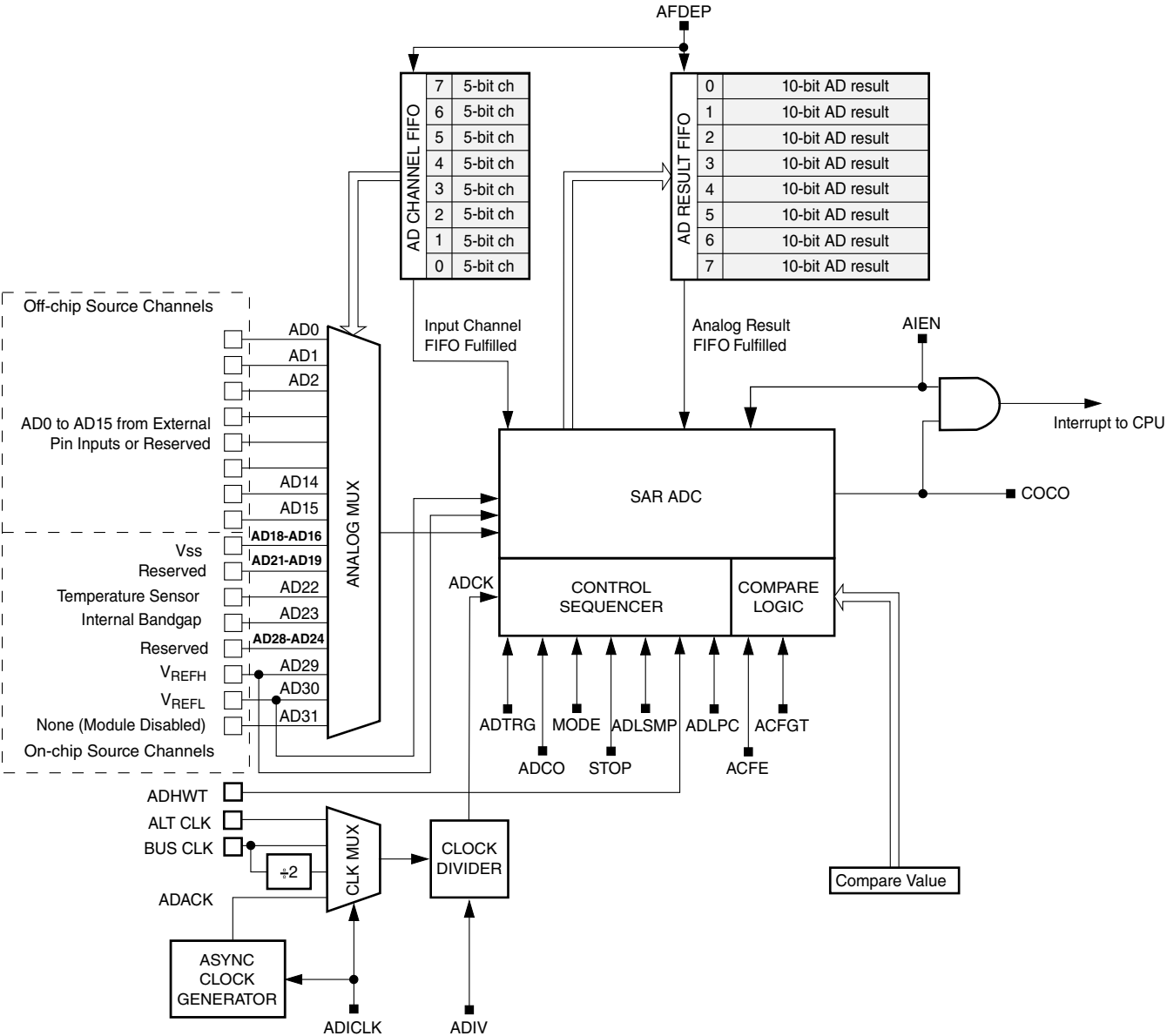
Figure 9-1. ADC block diagram
