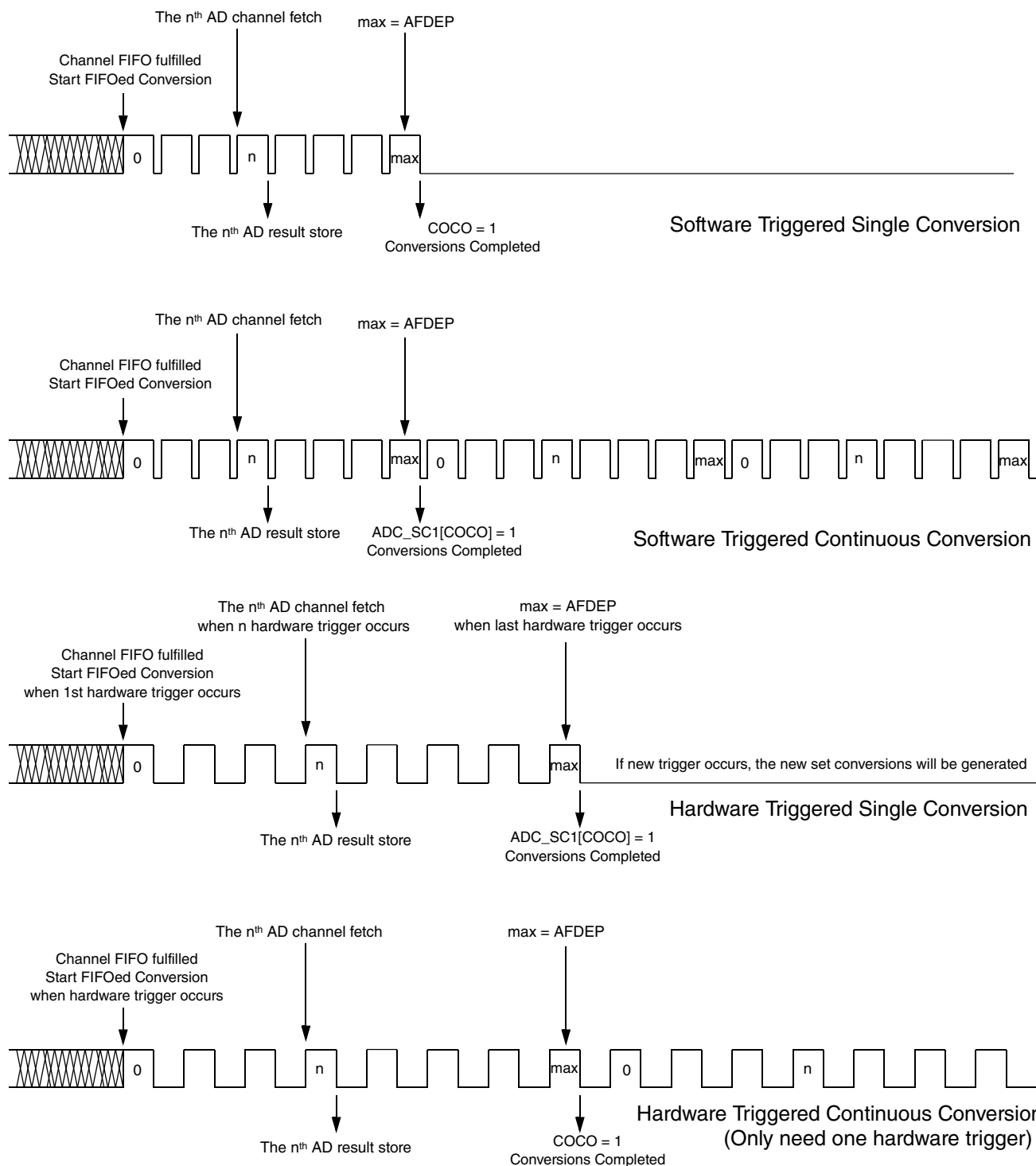
Figure 16-2. ADC FIFO conversion sequence
