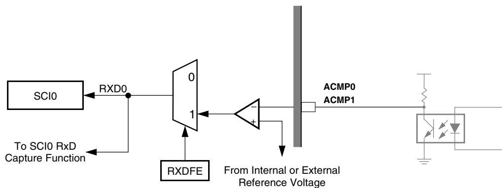
Figure 6-4. IR demodulation diagram
