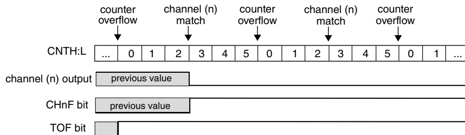
Figure 12-9. Example of the output compare mode when the match clears the channel output
