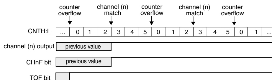
Figure 12-10. Example of the output compare mode when the match sets the channel output
