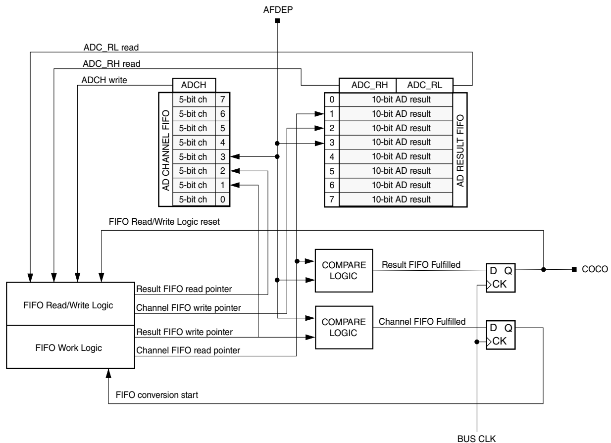
Figure 16-1. FADC FIFO structure
