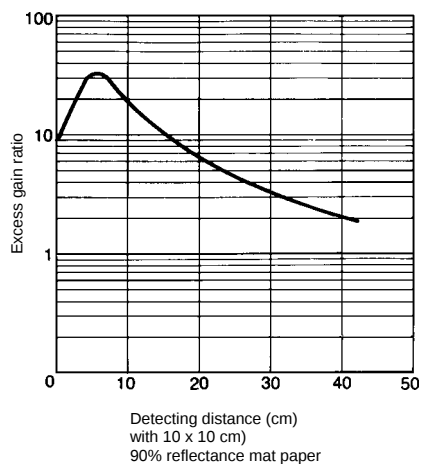
Diffuse reflective type (E3JK-DS30M□-US)
