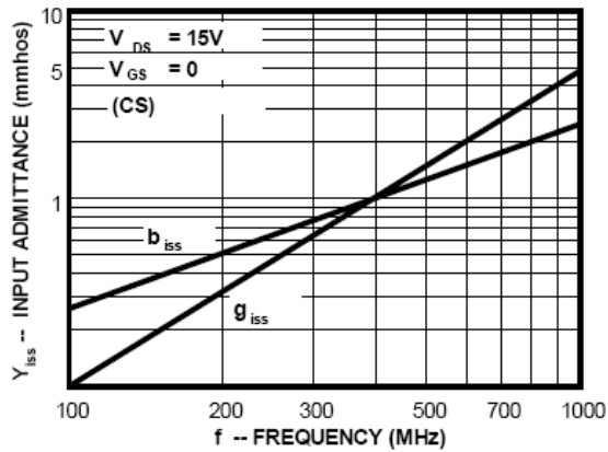
Input Admittance
