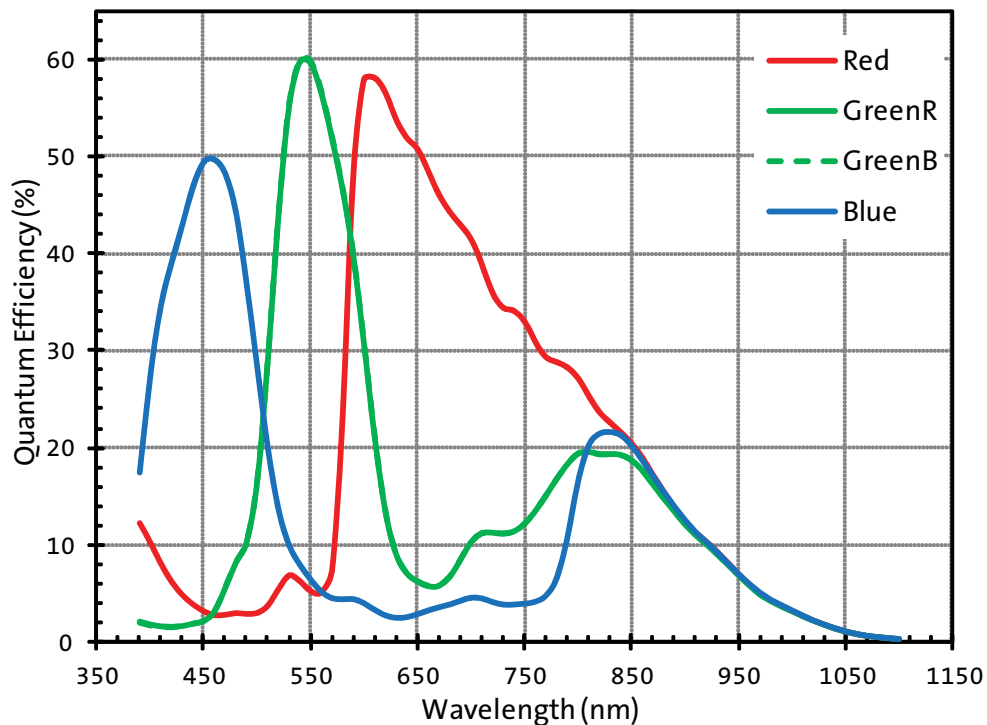
Figure 50: Quantum Efficiency
