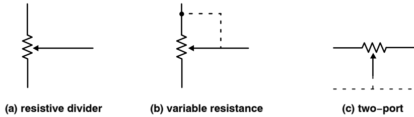
Figure 6. Potentiometer Configuration
