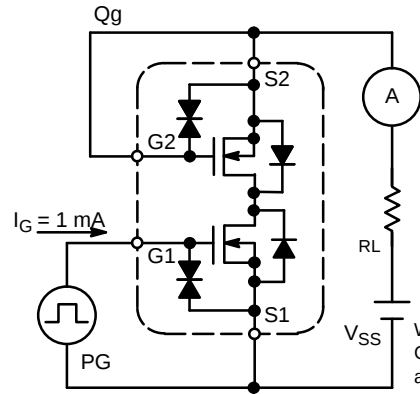
Figure 16. Test Circuit 6
