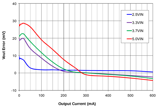
Figure 8. 1.82V OUT Regulation (Normalized)
