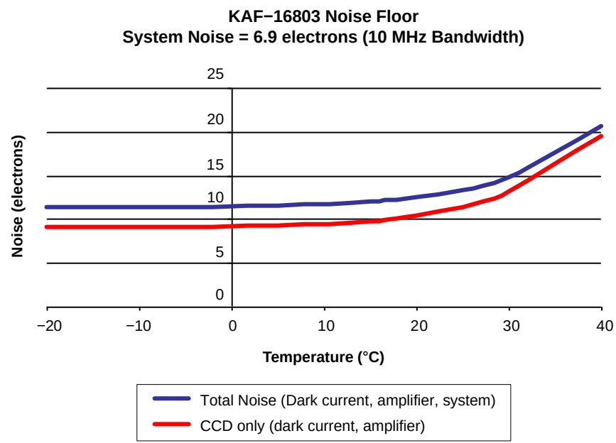
Figure 9. Noise Floor
