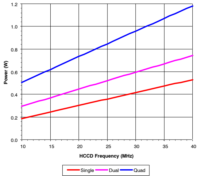
Figure 11. Power
