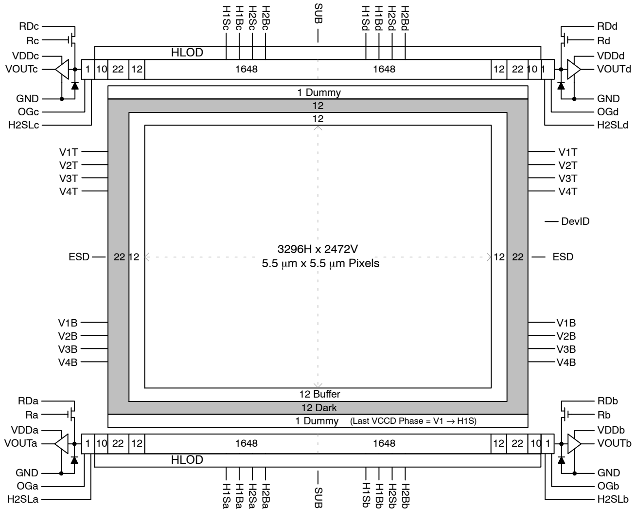
Figure 2. Block Diagram
