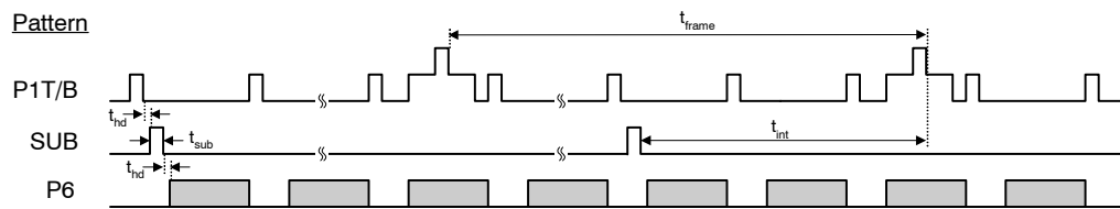
Figure 23. Frame/Electronic Shutter Timing
