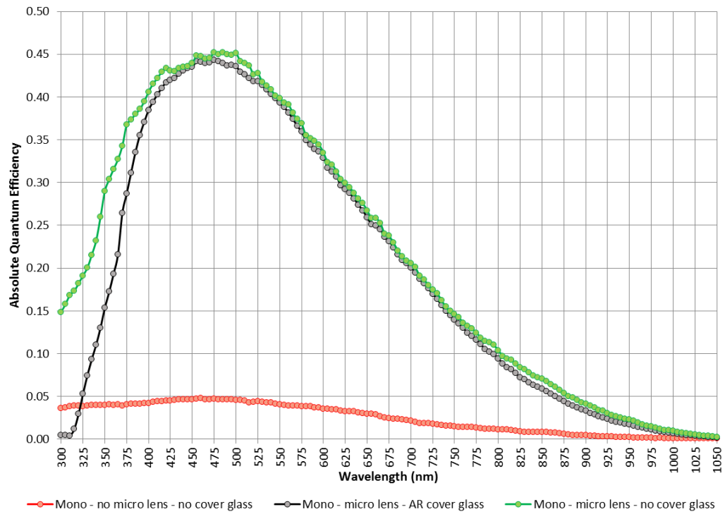
Figure 6. Monochrome Configurations – Quantum Efficiency
