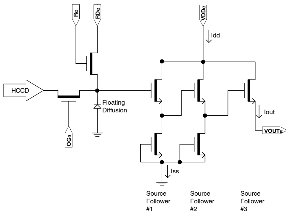
Figure 17. Output Amplifier
