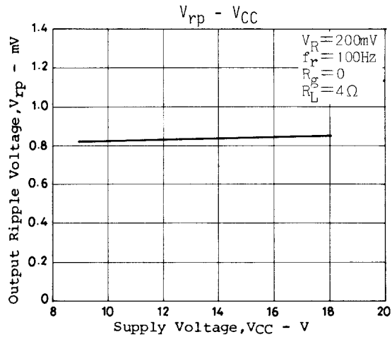
Figure 46. V_{rp} - V_{CC}
