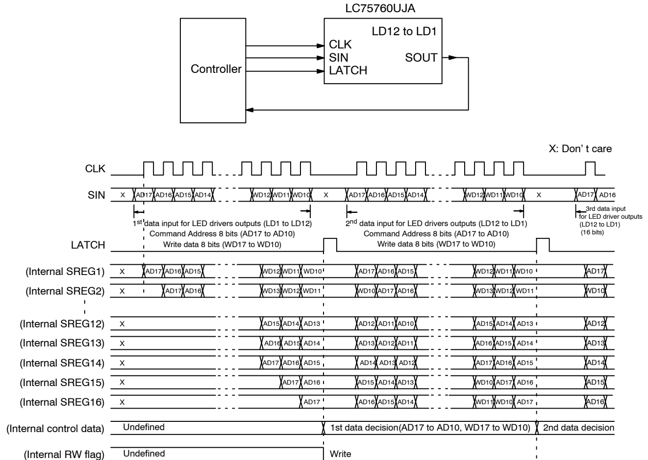
Figure 7. Transfer Example of Write Data of 4-line Serial Interface Using One Device
