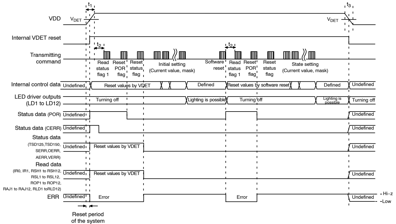
Figure 24. Reset Action Sequence (When \overline{RES} Pin is Used)
