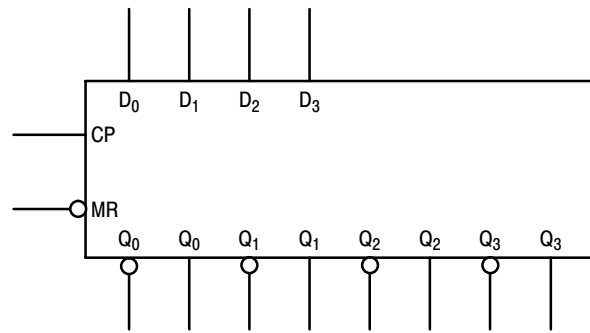
Figure 2. Logic Symbol
