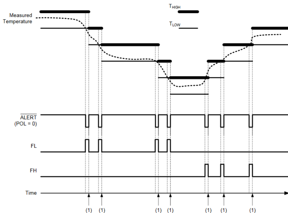
Figure 6. Interrupt Mode
