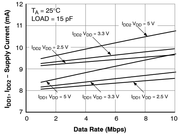
Figure 6. NCID9411 Supply Current vs. Data Rate (Load = 15\text{ pF} )
