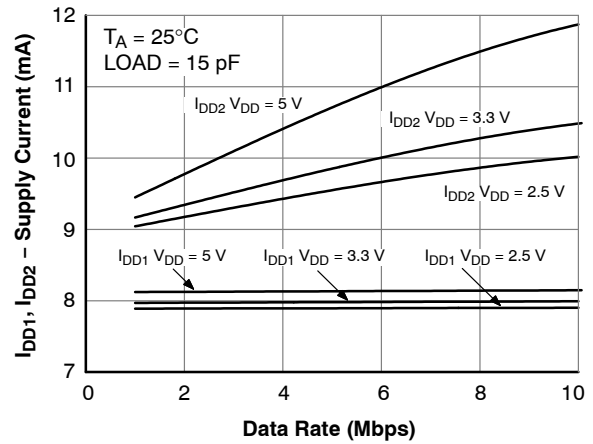
Figure 4. NCID9401 Supply Current vs. Data Rate (Load = 15\text{ pF} )
