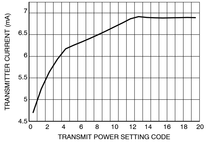
Figure 23. 1 V Mode Transmitter Current versus Power Setting
