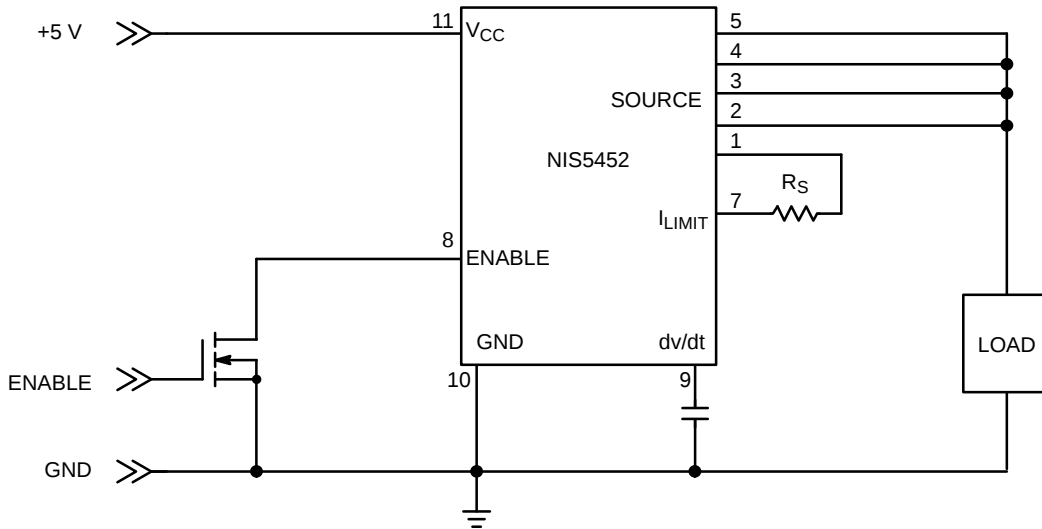
Figure 3. Application Circuit with Kelvin Current Sensing
