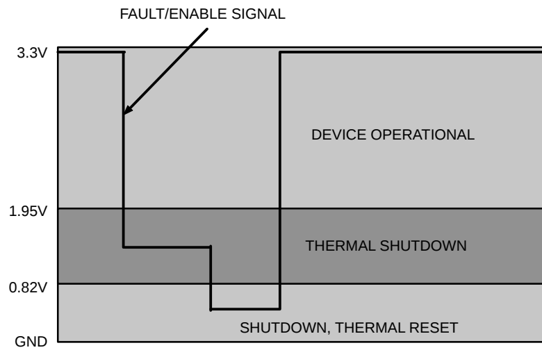
Figure 5. Enable/Fault Signal Levels
