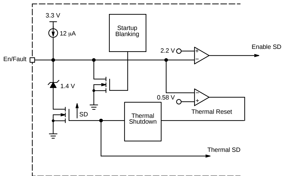
Figure 6. Enable/Fault Simplified Circuit
