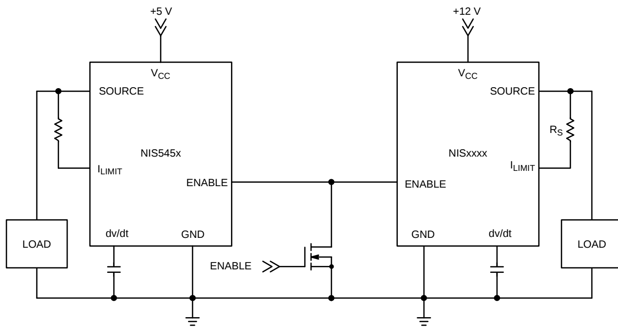
Figure 4. Common Thermal Shutdown
