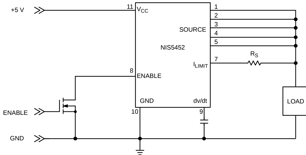
Figure 2. Application Circuit with Direct Current Sensing
