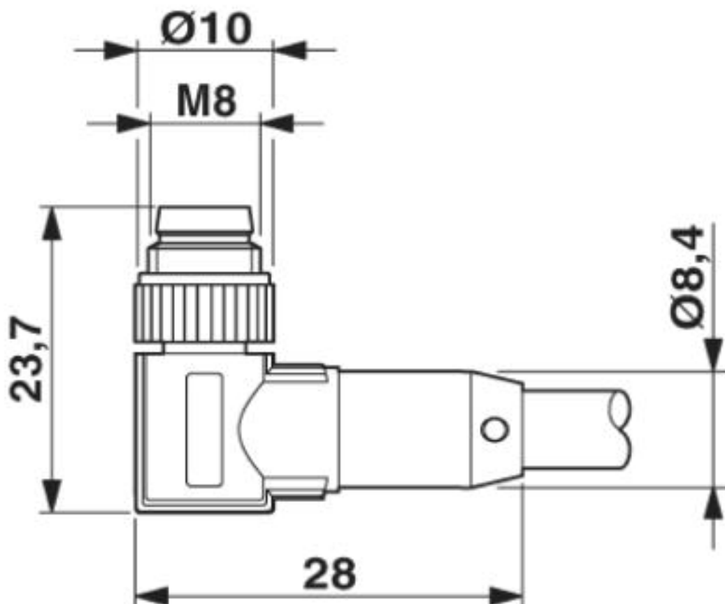
Dimensional drawing
