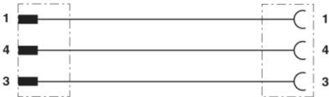
Contact assignment of M12 plugs / M8 sockets
