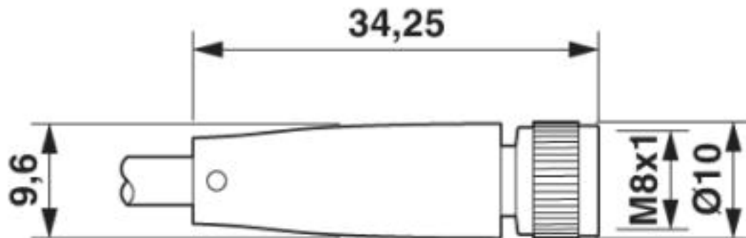
Dimensional drawing
