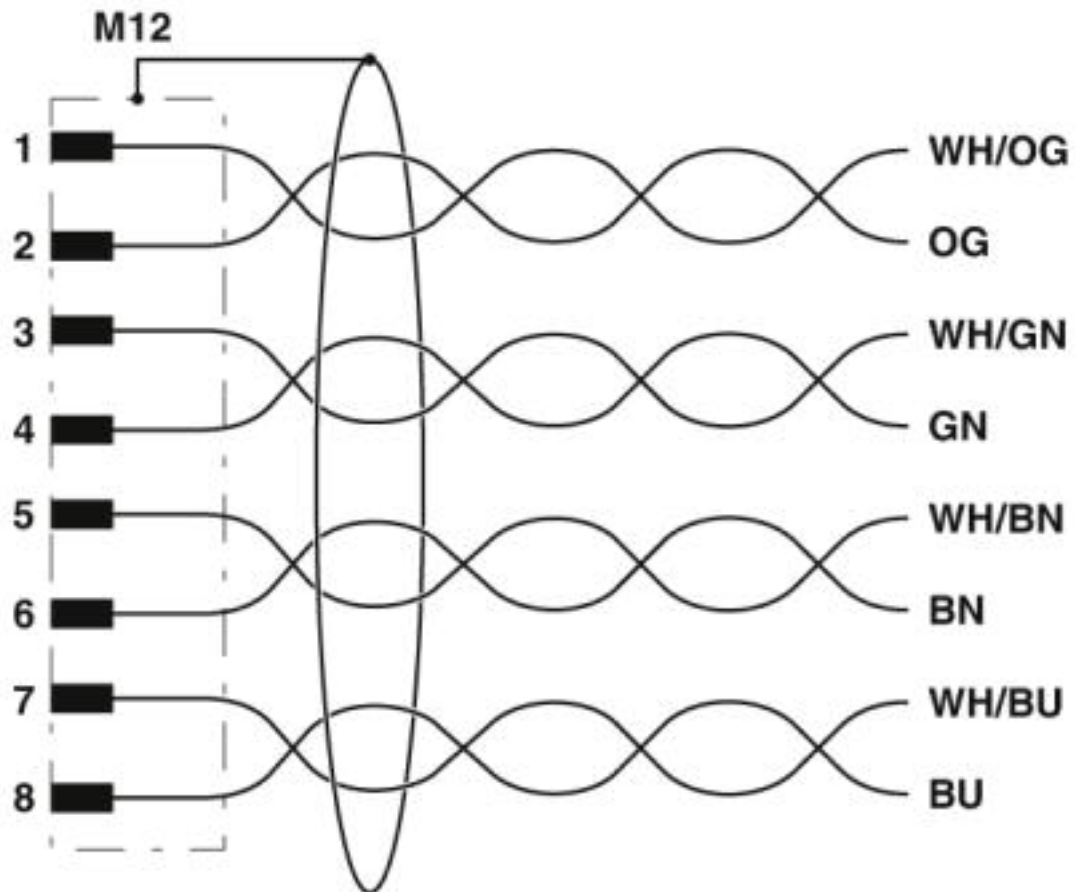
Circuit diagram
