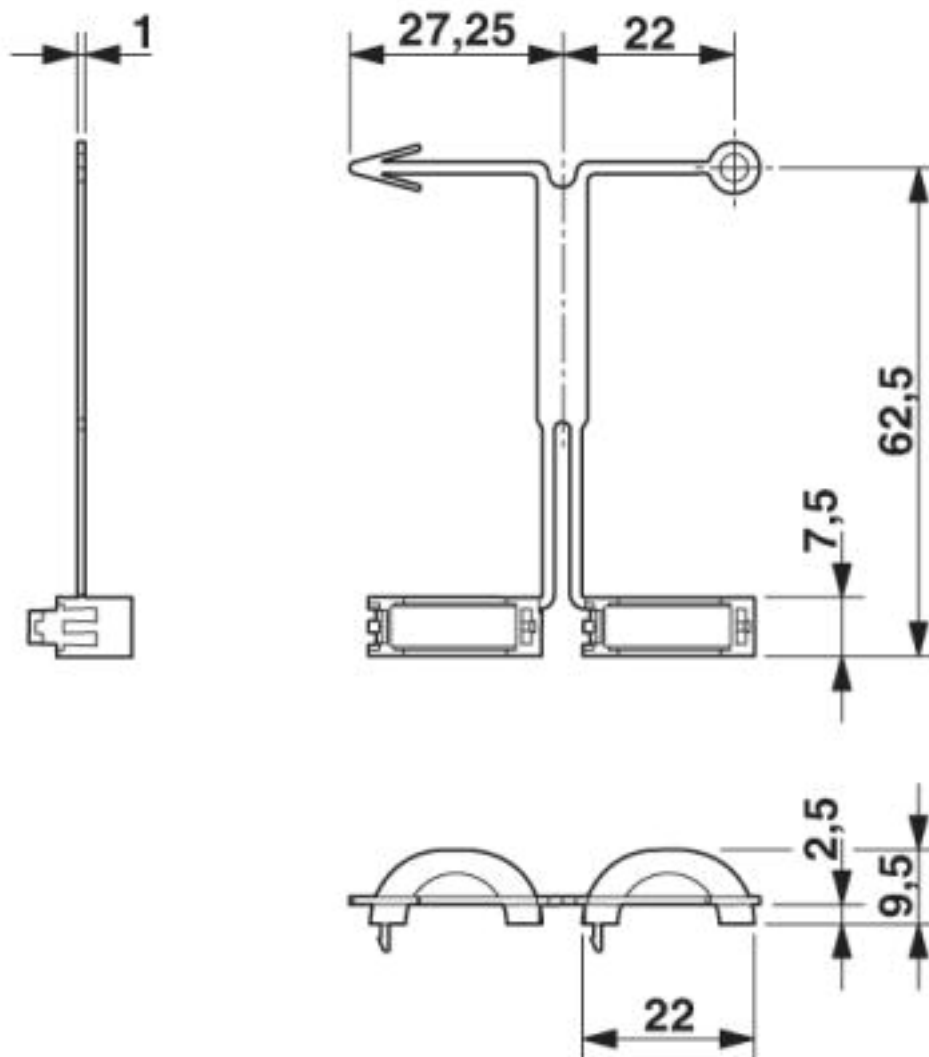
Dimensional drawing
