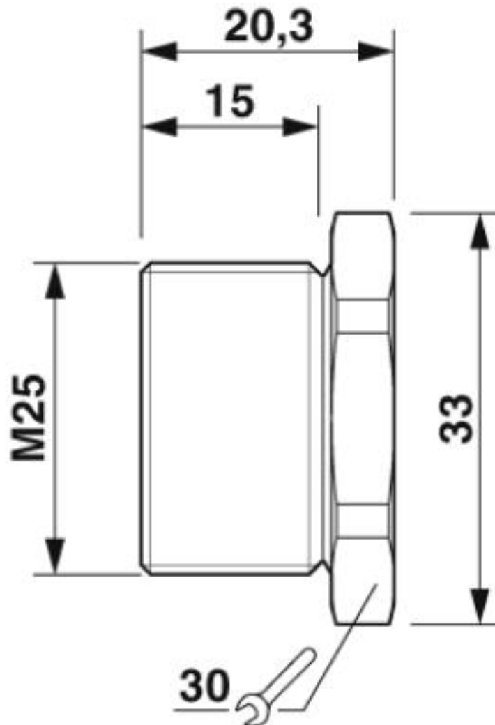
Dimensional drawing
