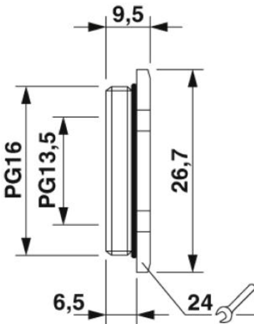
Dimensional drawing
