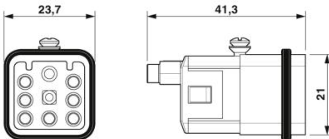
Male insert (turned contacts)
