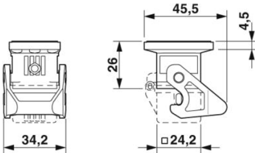
Dimensional drawing
