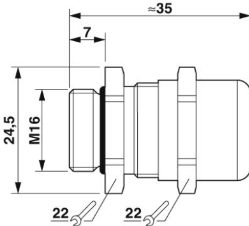
Dimensional drawing
