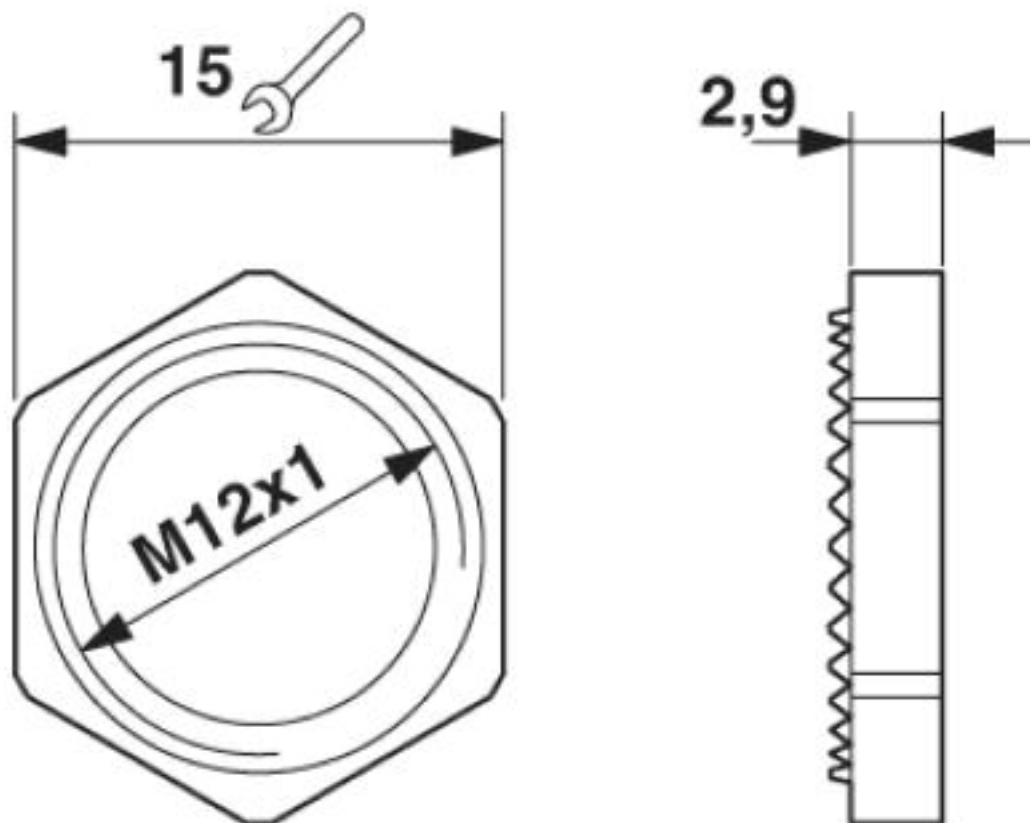
Dimensional drawing
