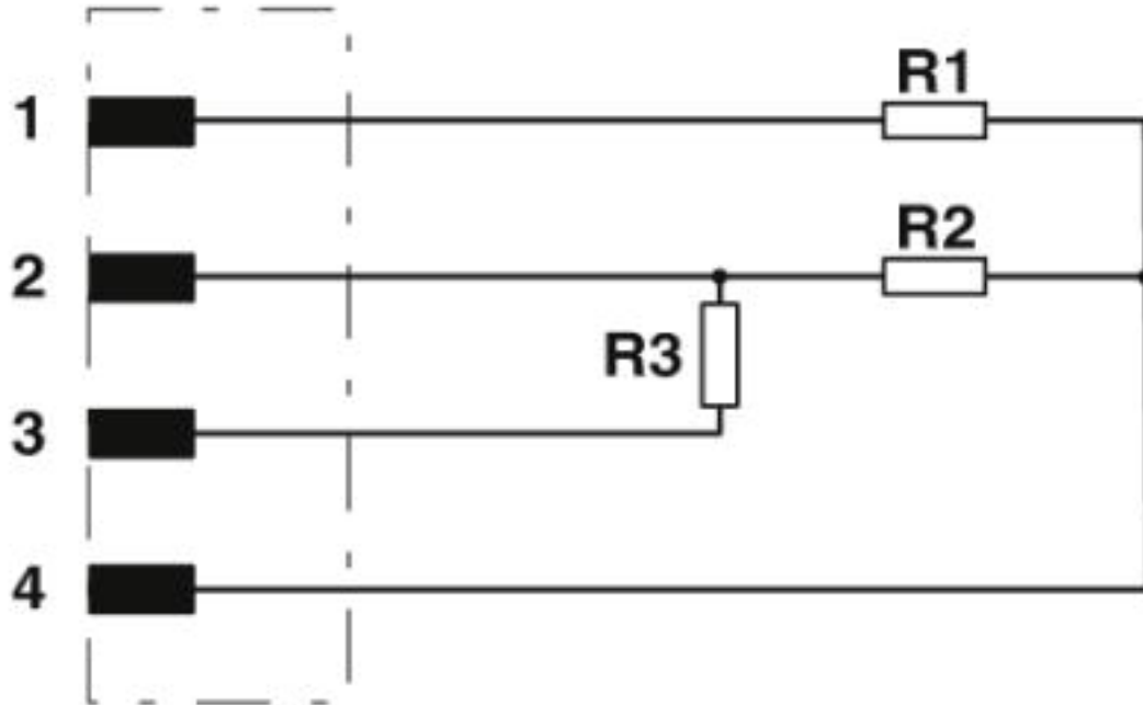
Circuit diagram
