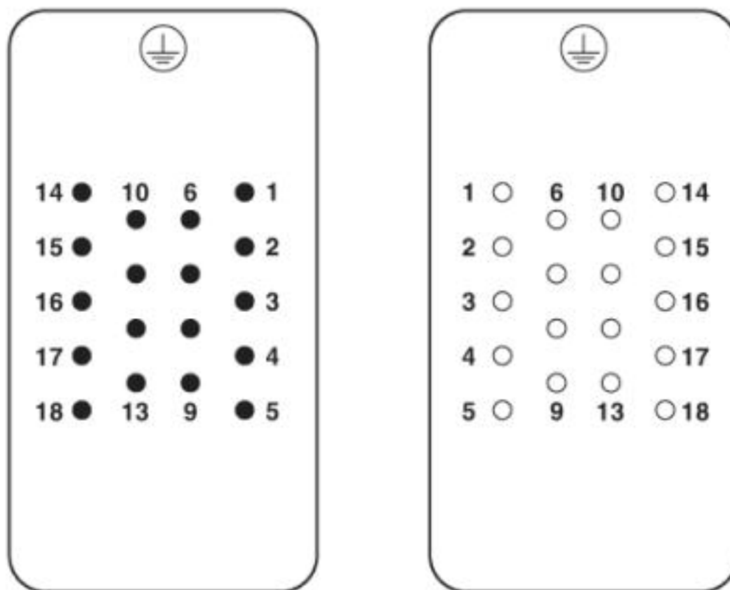
Schematic diagram
