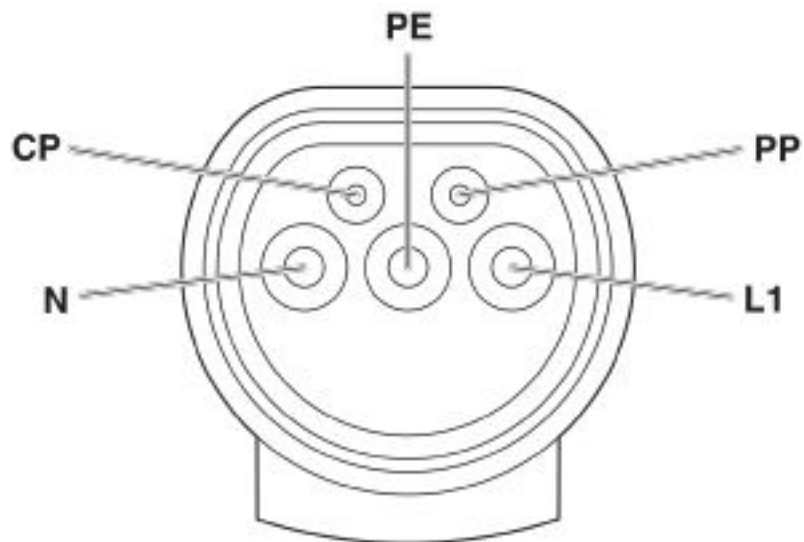
Schematic diagram
