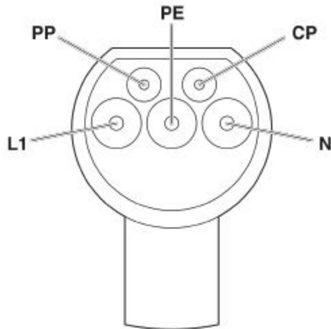
Connection diagram
