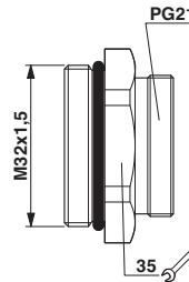
Dimensional drawing
