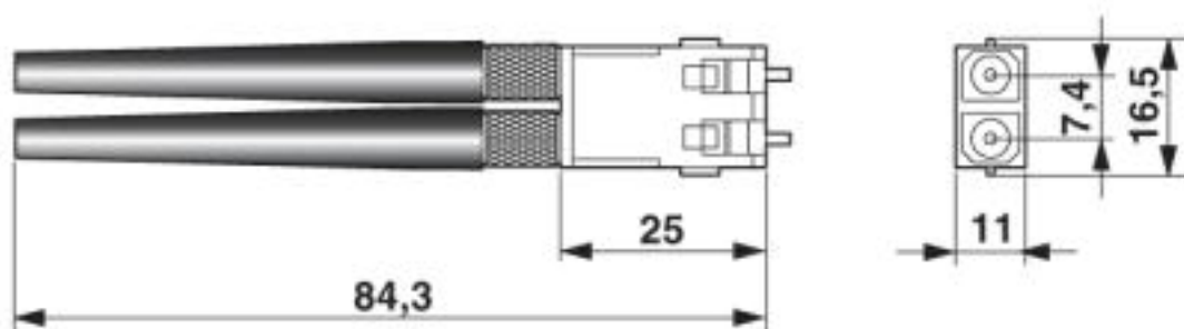
Dimensional drawing
