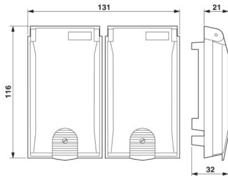
Mounting frame
