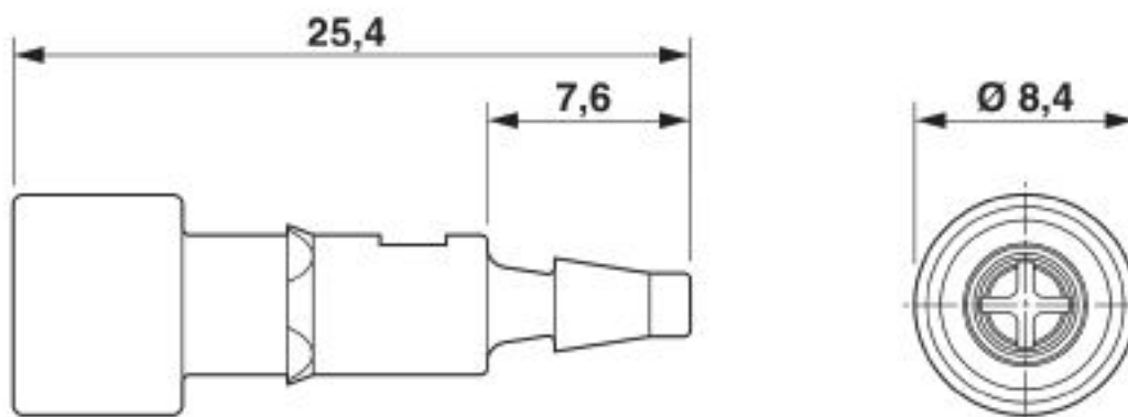
Dimensional drawing
