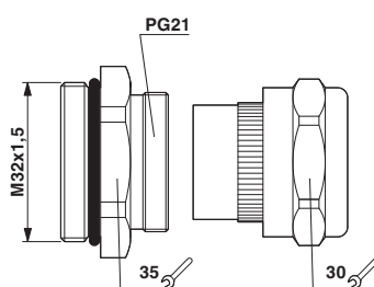
Dimensional drawing
