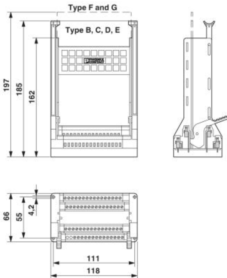
Dimensional drawing
