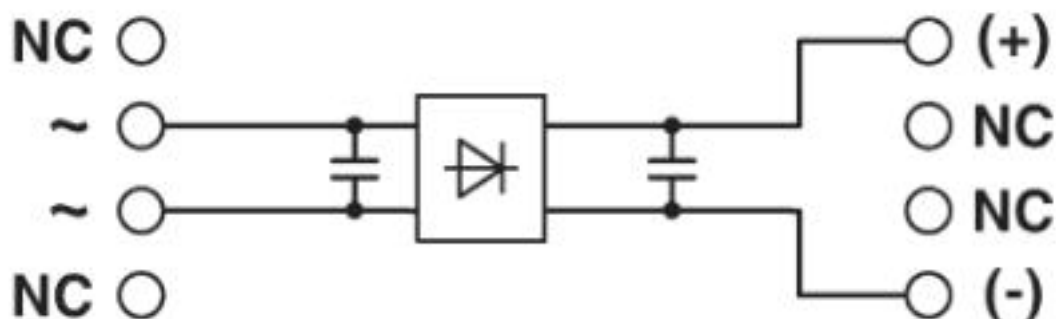
Block diagram
