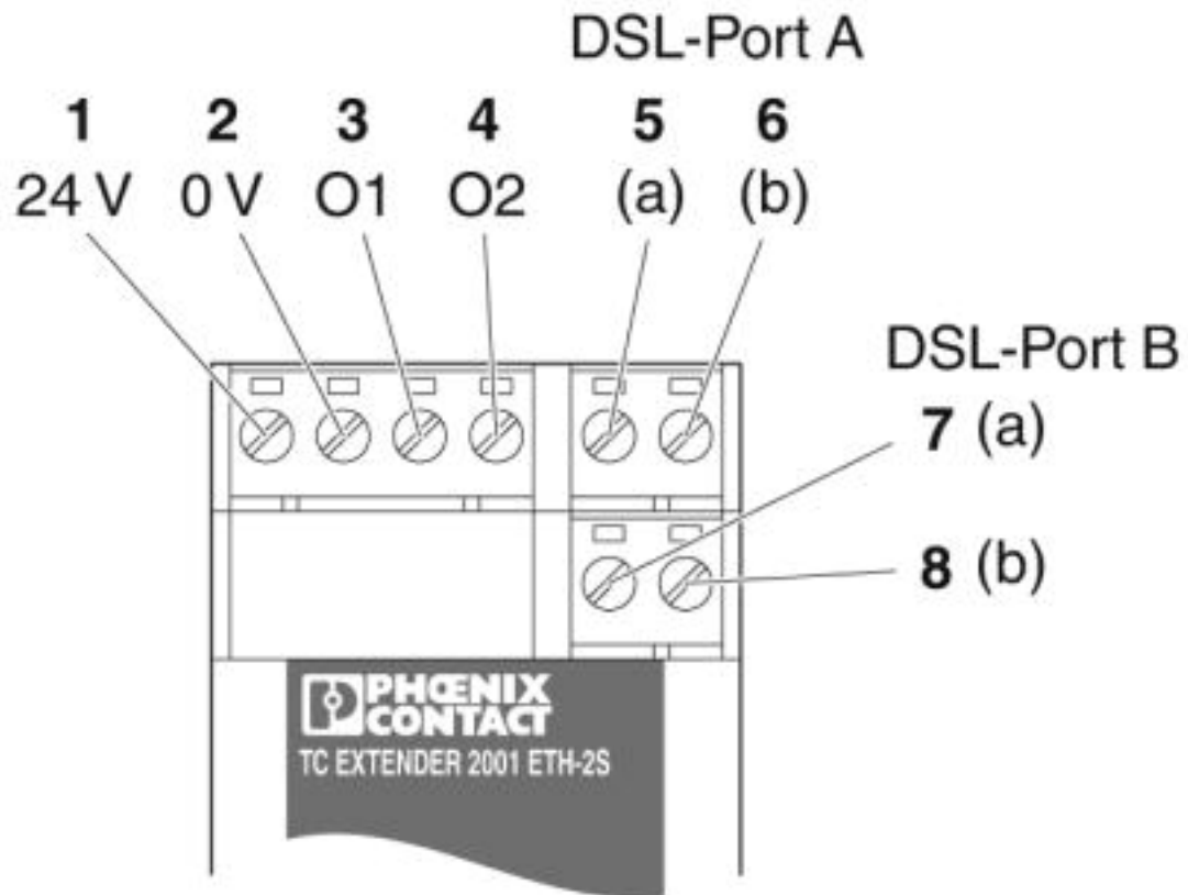
Schematic diagram
