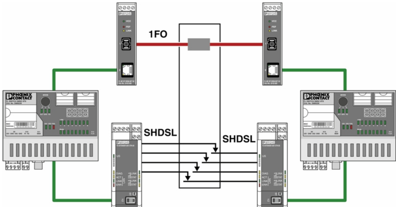
Application drawing
