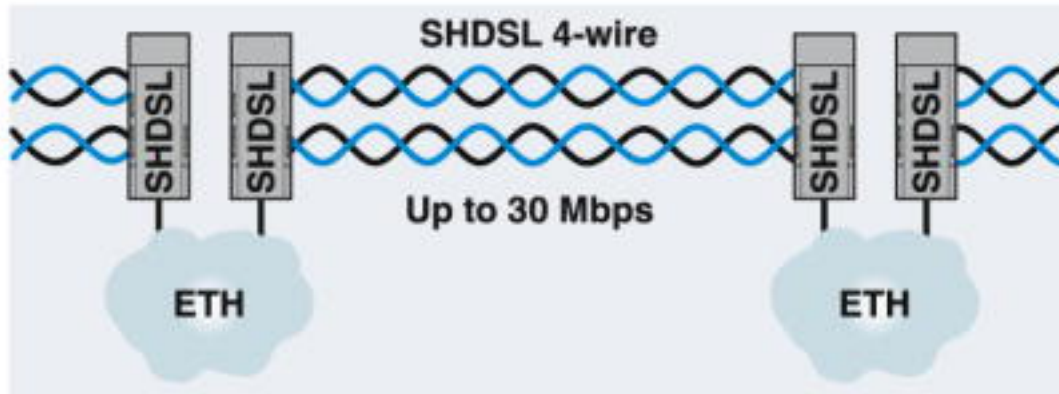
Application drawing
