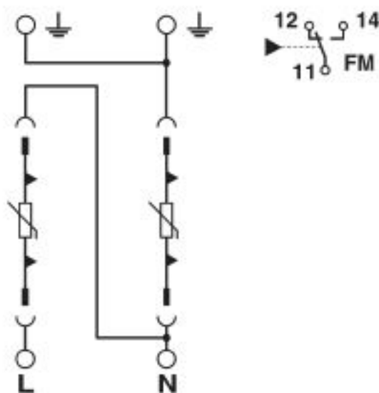
Circuit diagram
