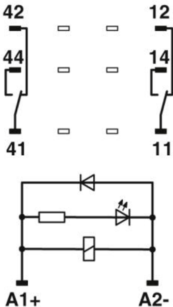
Circuit diagram
