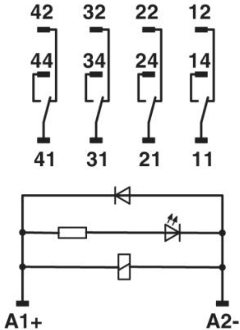
Circuit diagram
