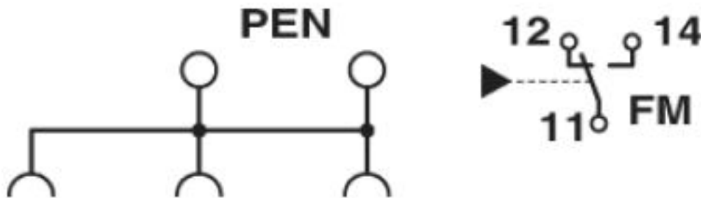
Circuit diagram
