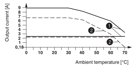
Derating curve ELR H5-ES-SC-24DC/500AC-2 and ELR H5-ES-SC-230AC/500AC-9 100% operating time
